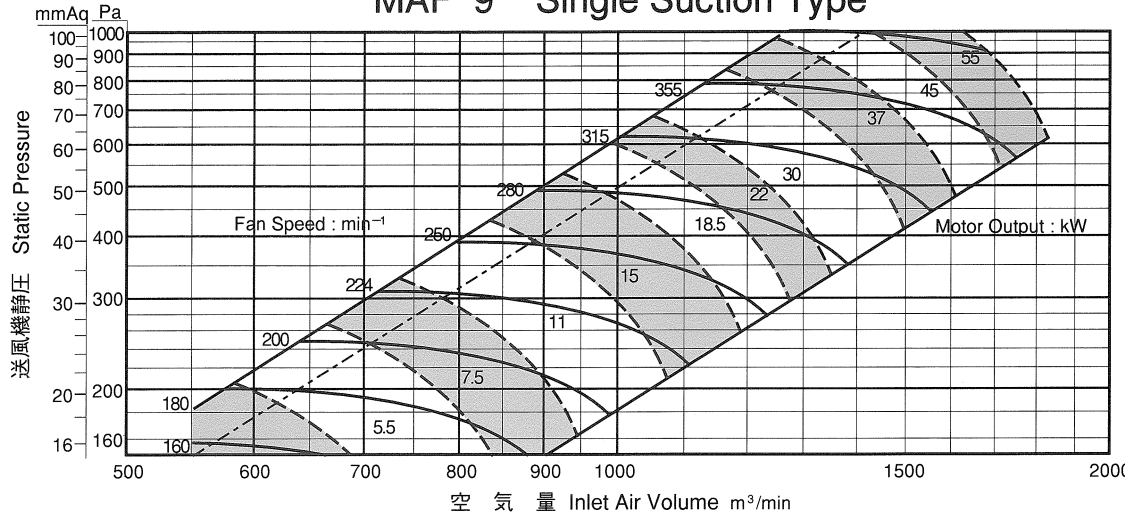
MAF 9 Single Suction Type
