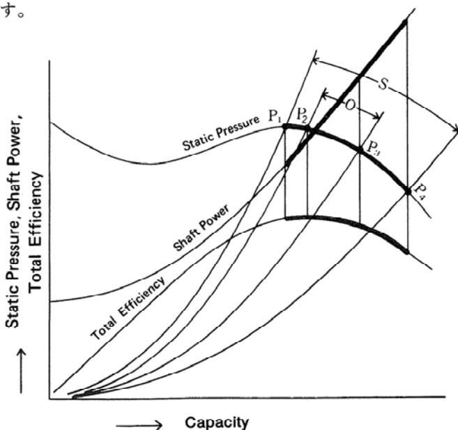
MAF 多翼送風機の特性と標準容量範囲の説明図 Characteristics and Standard Capacity Range of MAF Multi-Blade Fan
